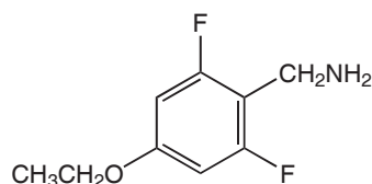
H32007 4-Ethoxy-2,6-difluorobenzylamine, 97%
