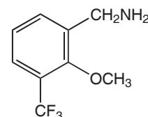
H32993 2-Methoxy-3-(trifluoromethyl)benzylamine, 97%
