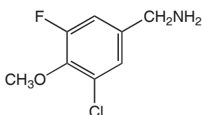
H31630 3-Chloro-5-fluoro-4-methoxybenzylamine, 97%
