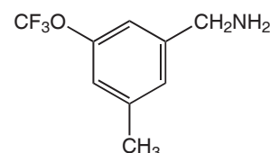
H31840 3-Methyl-5-(trifluoromethoxy)benzylamine, 97%
