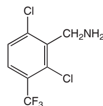
H31539 2,6-Dichloro-3-(trifluoromethyl)benzylamine, 97%
